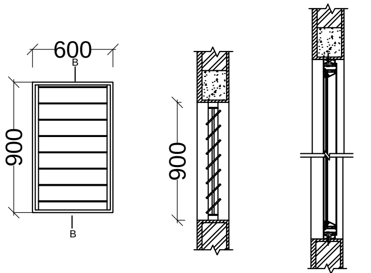
WINDOW TYPE W4 (LOUVERS)
