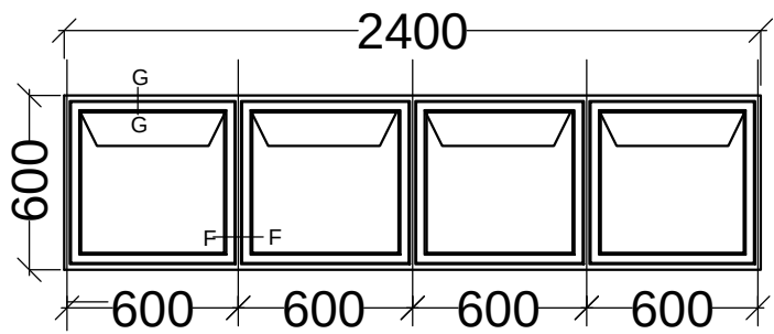
WINDOW TYPE W
