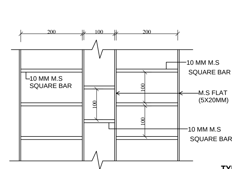
TYPICAL WINDOW AND VENTILATOR GRILL DETAIL
