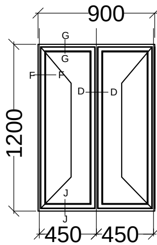
WINDOW TYPE W3V3
