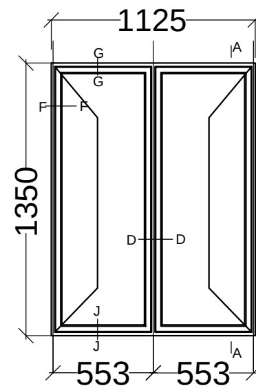
WINDOW TYPE W2V2
